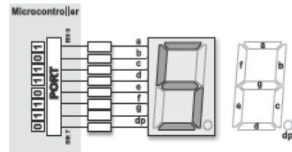
Port and LED display connection
